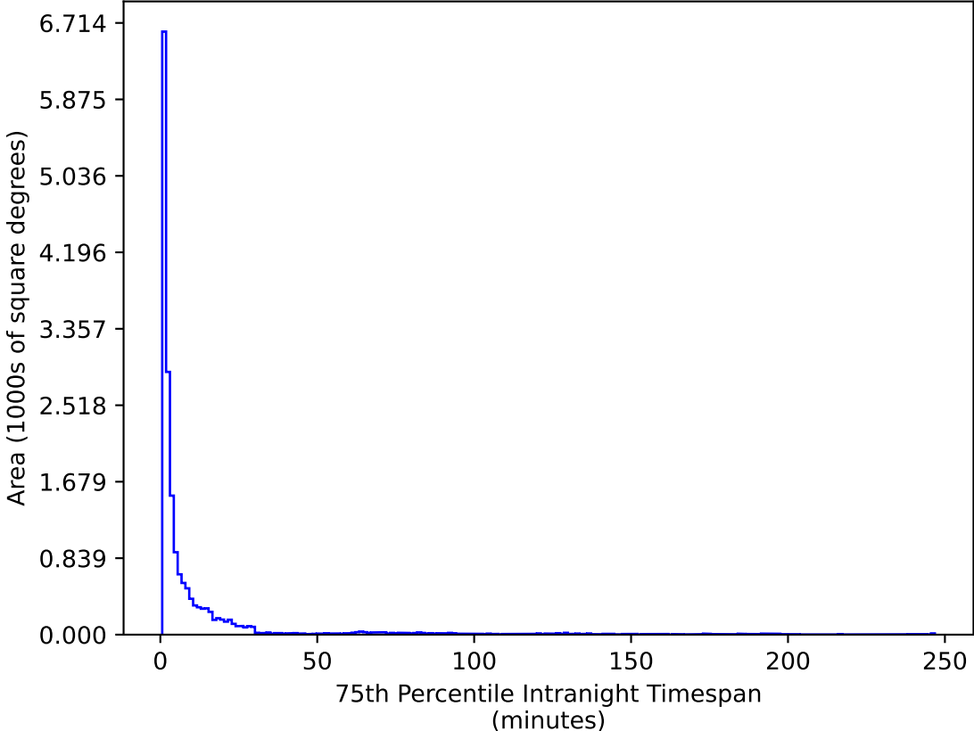
ddf_acor_sf15_lsf40_lsr10_v3.4_10yrs WFD u band: 75th Percentile Intranight Timespan
