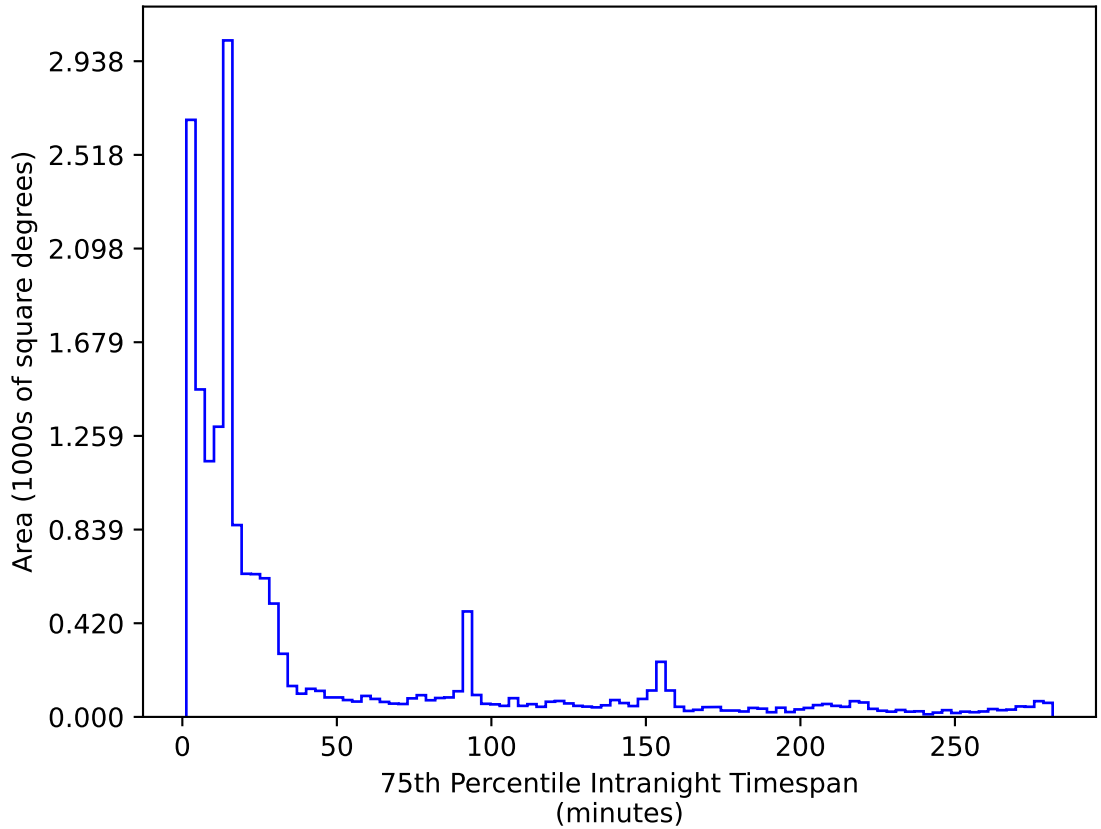
ddf_acor_sf15_ls40_lsr10_v3.4_10yrs WFD r band: 75th Percentile Intranight Timespan
