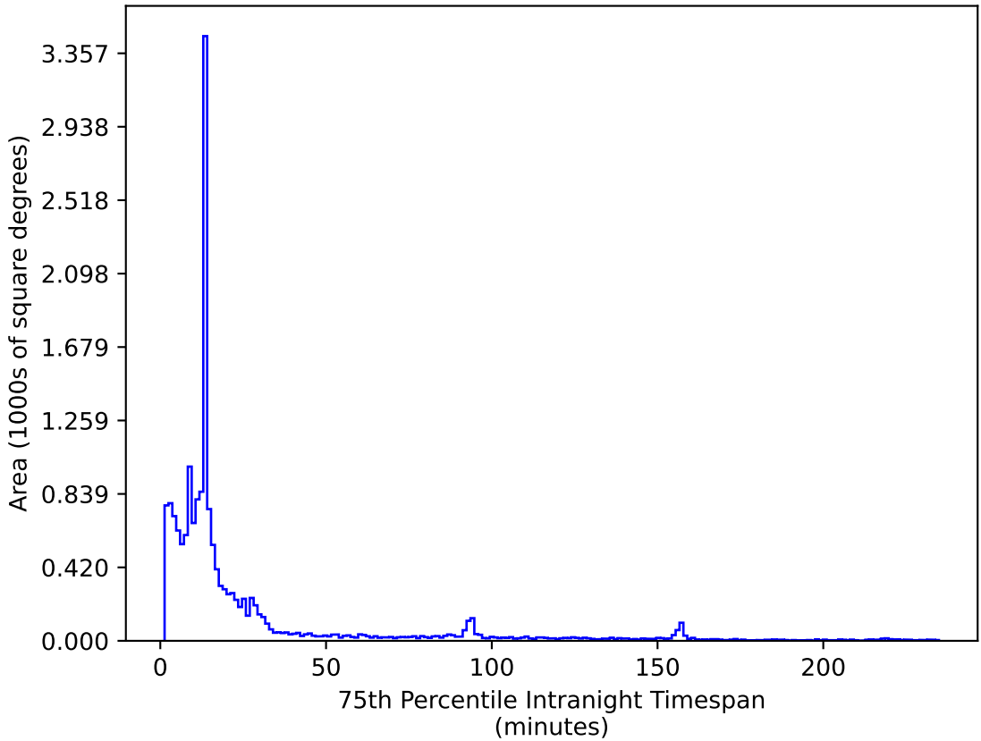
ddf_acor_sf15_lsf40_lsr10_v3.4_10yrs WFD i band: 75th Percentile Intranight Timespan
