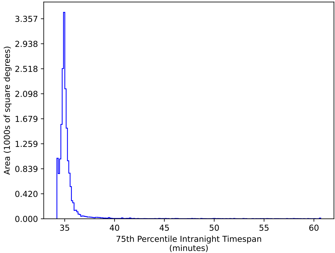
ddf_acor_sf15_lsf40_lsr10_v3.4_10yrs WFD gr bands: 75th Percentile Intranight Timespan
