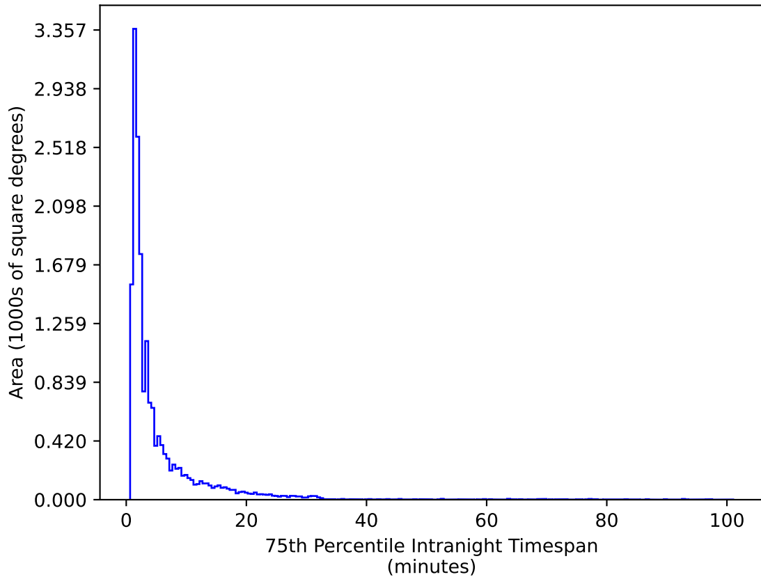
ddf_acor_sf15_lsf40_lsr10_v3.4_10yrs WFD g band: 75th Percentile Intranight Timespan
