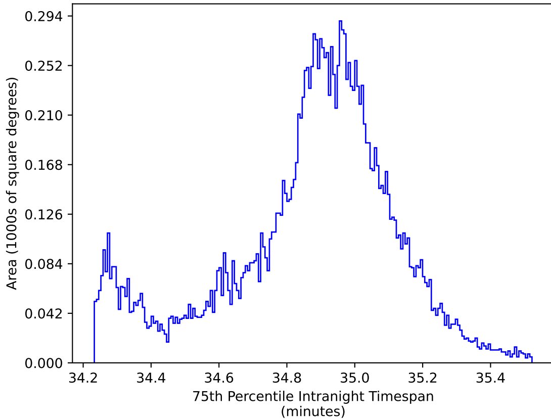
ddf_acor_sf15_lsf40_lsr10_v3.4_10yrs WFD all bands: 75th Percentile Intranight Timespan
