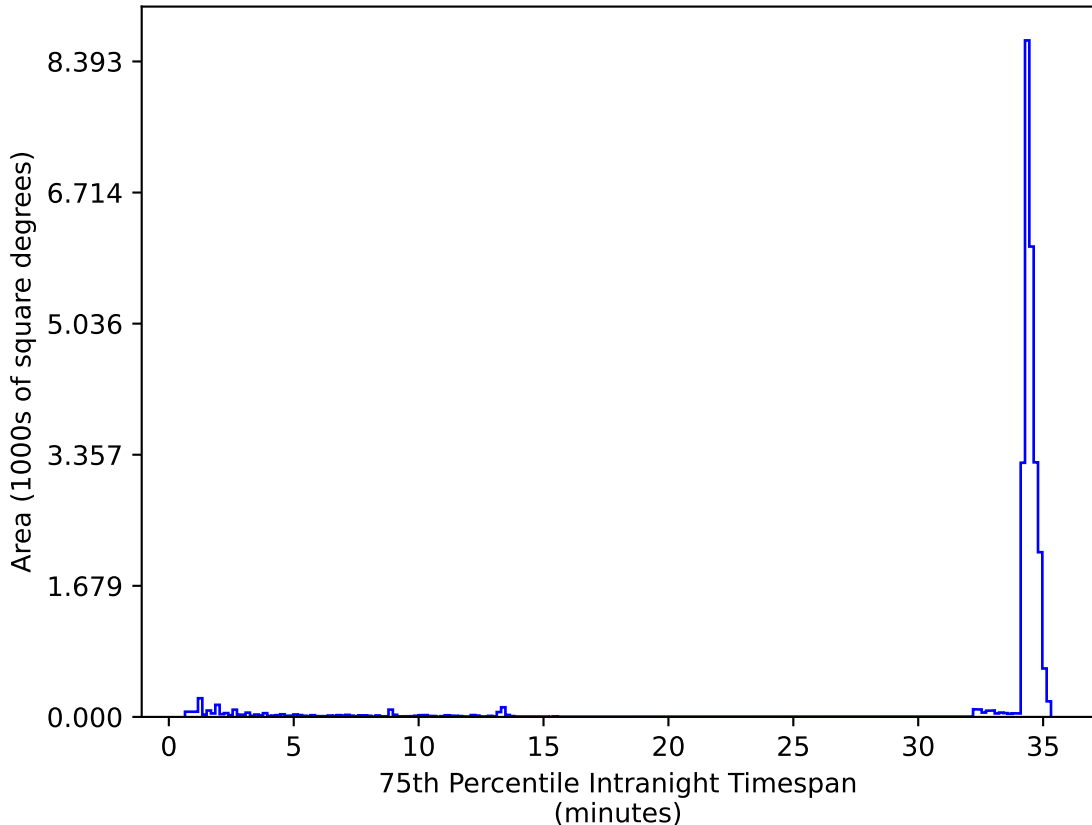
ddf_acor_sf15_lsf40_lsr10_v3.4_10yrs All sky zy bands: 75th Percentile Intranight Timespan
