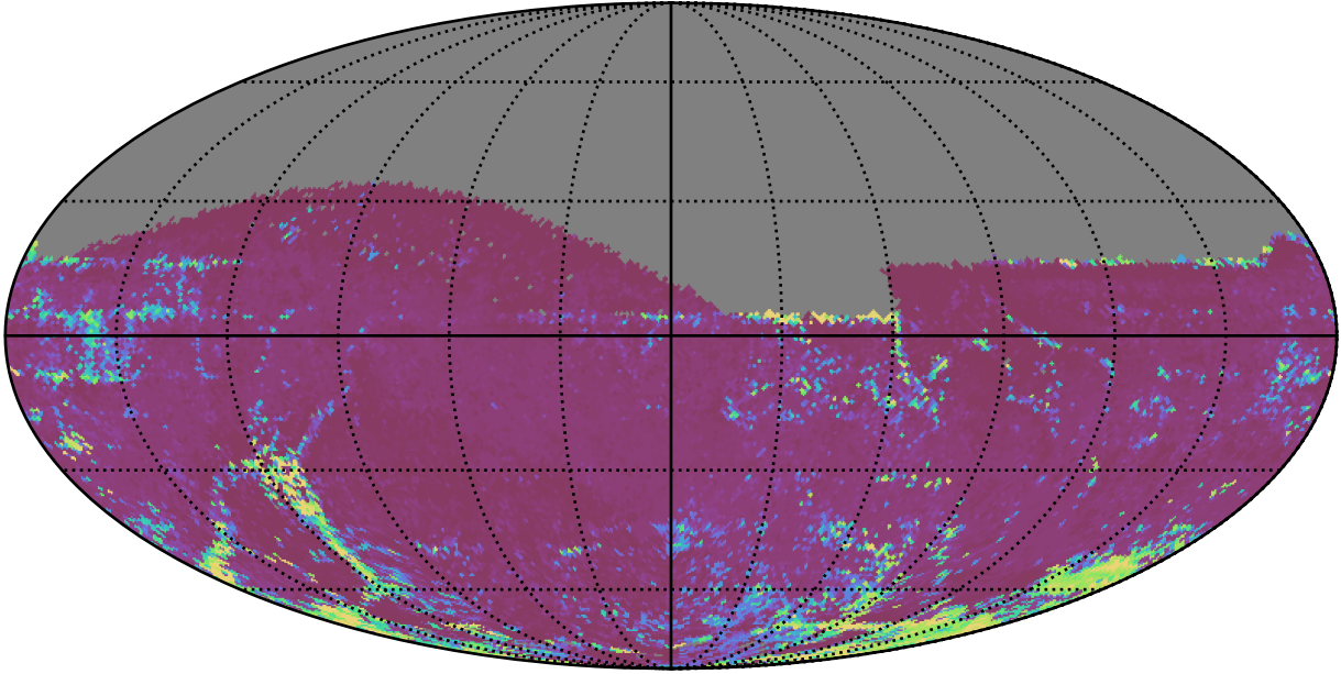
ddf_acor_sf15_lsf40_lsr10_v3.4_10yrs All sky z band: 75th Percentile Intranight Timespan
