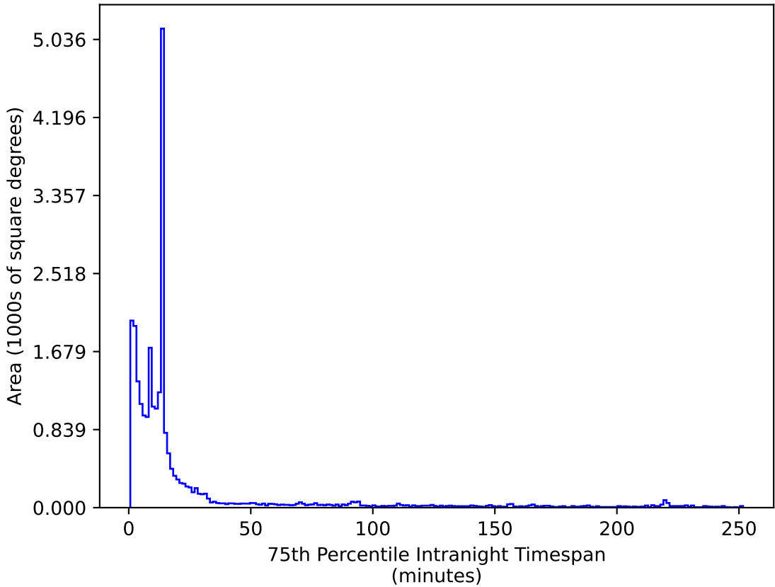
ddf_acor_sf15_lsf40_lsr10_v3.4_10yrs All sky z band: 75th Percentile Intranight Timespan
