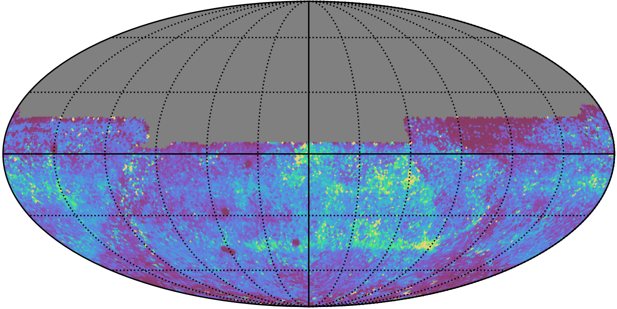
ddf_acor_sf15_lsf40_lsr10_v3.4_10yrs All sky y band: 75th Percentile Intranight Timespan
