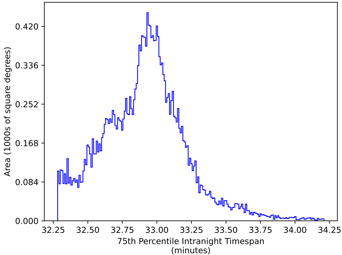
ddf_acor_sf15_ls40_lsr10_v3.4_10yrs All sky y band: 75th Percentile Intranight Timespan
