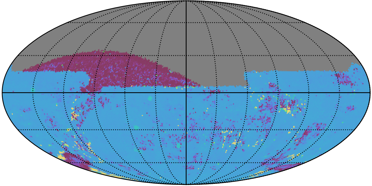
ddf_acor_sf15_lsf40_lsr10_v3.4_10yrs All sky ug bands: 75th Percentile Intranight Timespan
