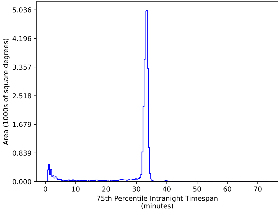
ddf_acor_sf15_lsf40_lsr10_v3.4_10yrs All sky ug bands: 75th Percentile Intranight Timespan
