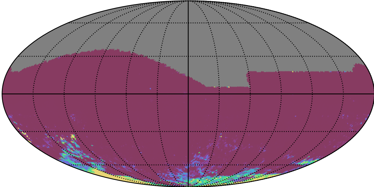
ddf_acor_sf15_lsf40_lsr10_v3.4_10yrs All sky ri bands: 75th Percentile Intranight Timespan
