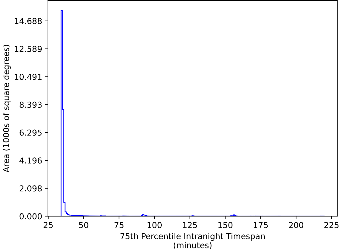
ddf_acor_sf15_lsf40_lsr10_v3.4_10yrs All sky ri bands: 75th Percentile Intranight Timespan
