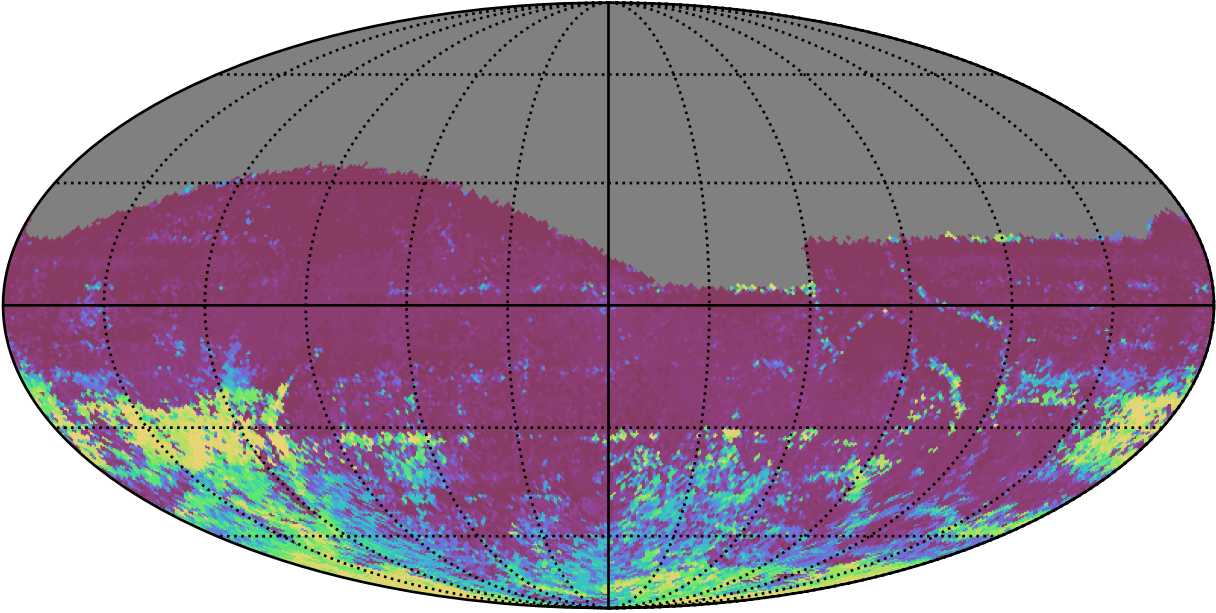
ddf_acor_sf15_ls40_lsr10_v3.4_10yrs All sky r band: 75th Percentile Intranight Timespan
