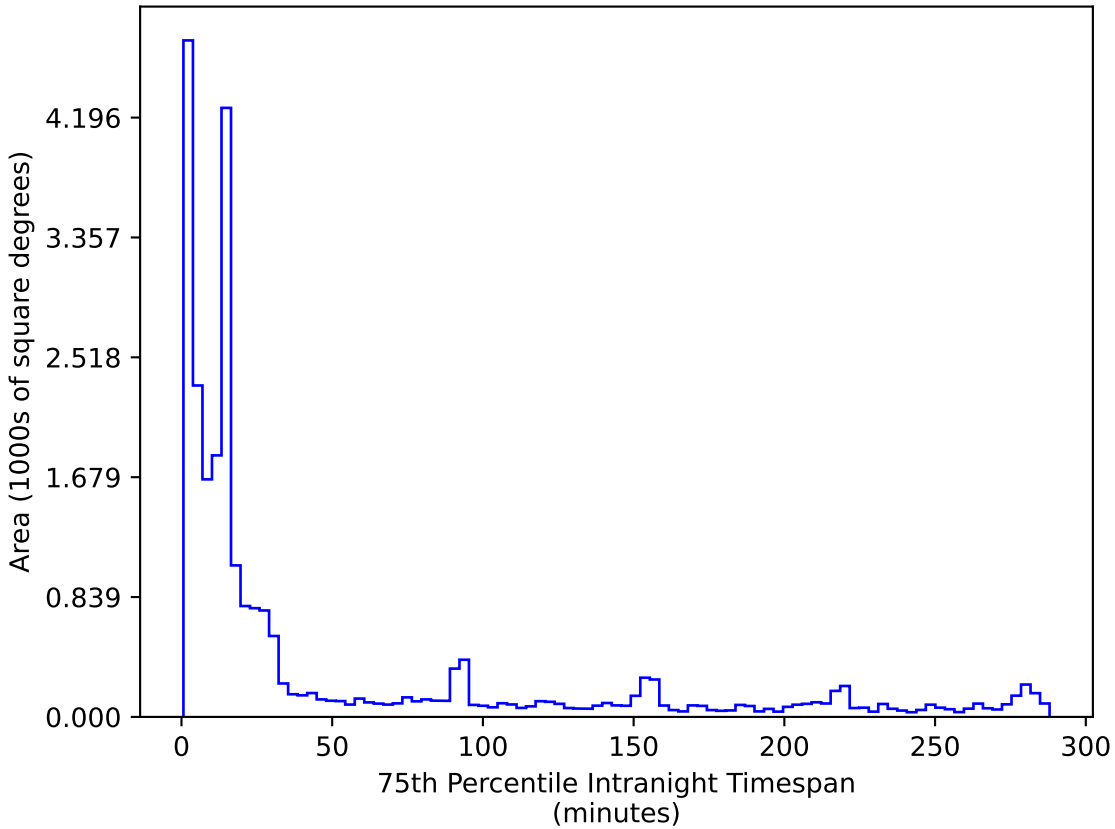
ddf_acor_sf15_lsf40_lsr10_v3.4_10yrs All sky r band: 75th Percentile Intranight Timespan
