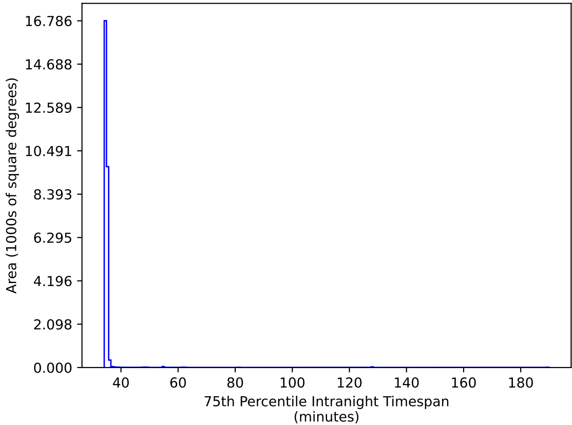
ddf_acor_sf15_lsf40_lsr10_v3.4_10yrs All sky iz bands: 75th Percentile Intranight Timespan
