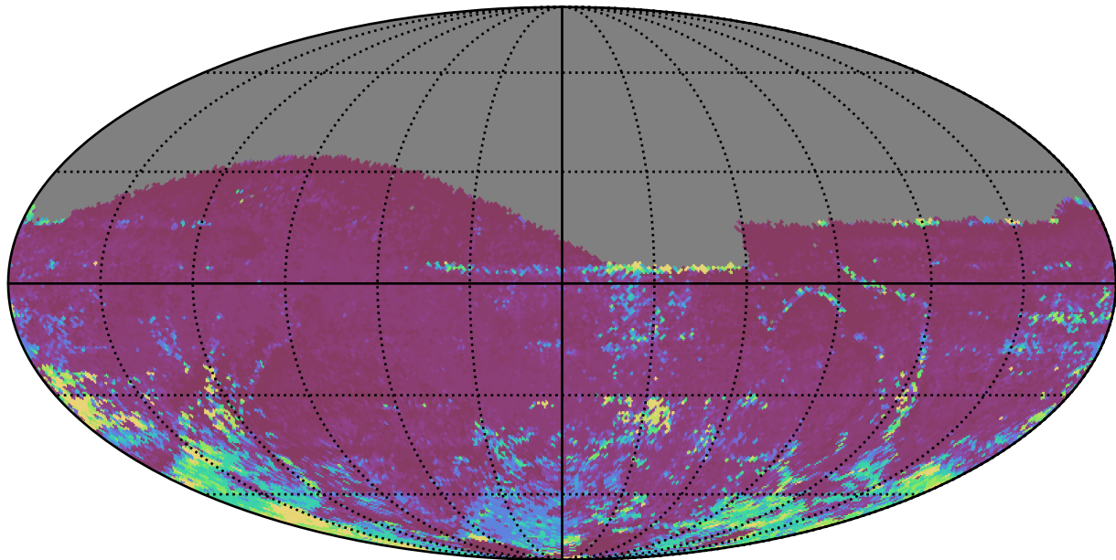
ddf_acor_sf15_lsf40_lsr10_v3.4_10yrs All sky i band: 75th Percentile Intranight Timespan
