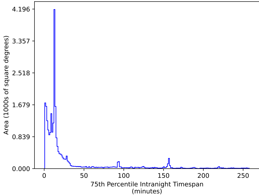
ddf_acor_sf15_lsf40_lsr10_v3.4_10yrs All sky i band: 75th Percentile Intranight Timespan
