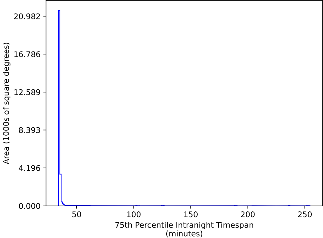
ddf_acor_sf15_lsf40_lsr10_v3.4_10yrs All sky gr bands: 75th Percentile Intranight Timespan
