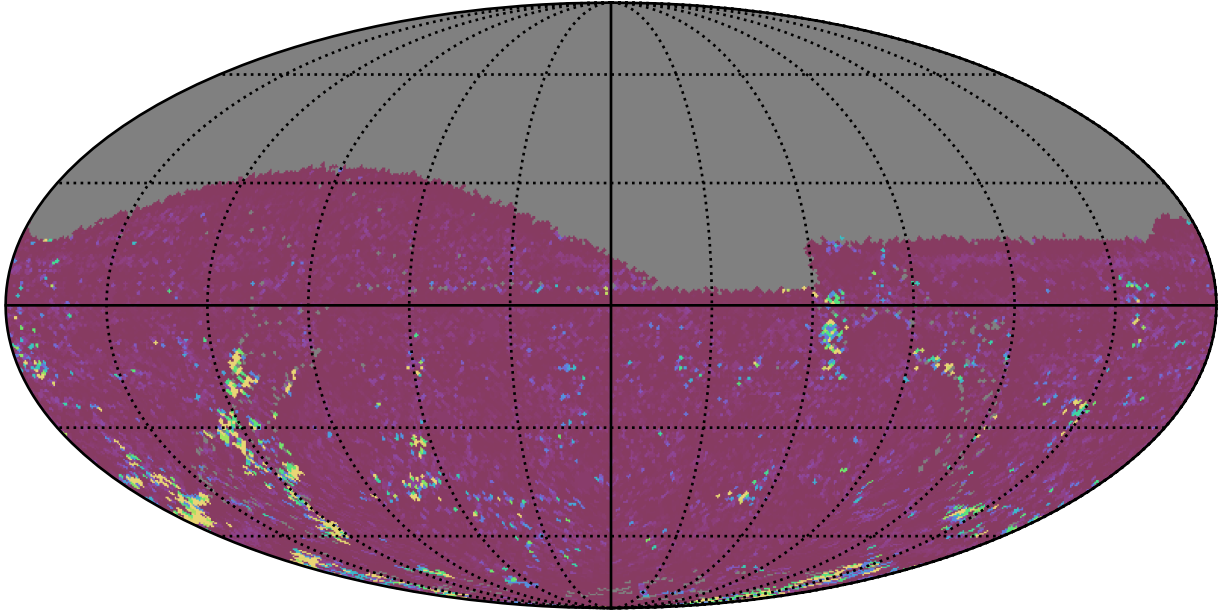
ddf_acor_sf15_lsf40_lsr10_v3.4_10yrs All sky g band: 75th Percentile Intranight Timespan
