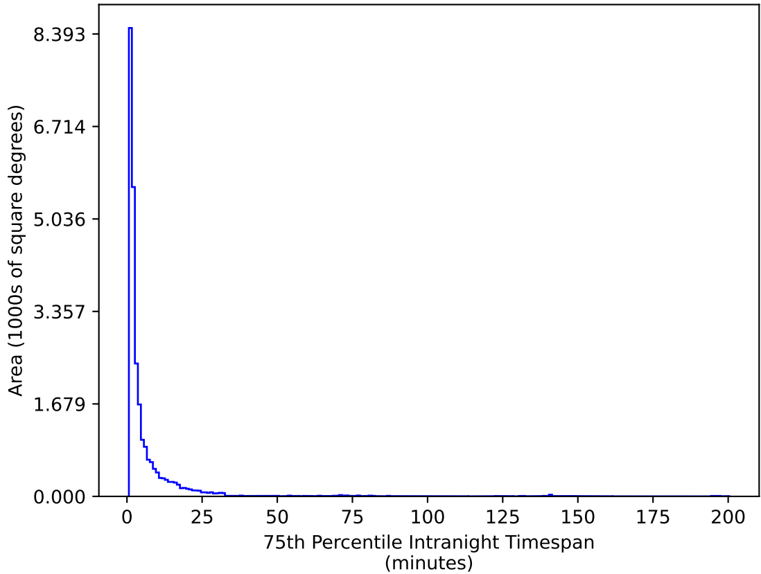
ddf_acor_sf15_lsf40_lsr10_v3.4_10yrs All sky g band: 75th Percentile Intranight Timespan
