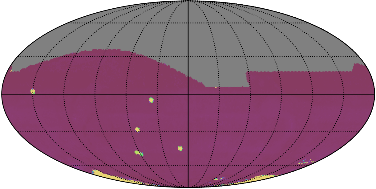
ddf_acor_sf15_lsf40_lsr10_v3.4_10yrs All sky all bands: 75th Percentile Intranight Timespan
