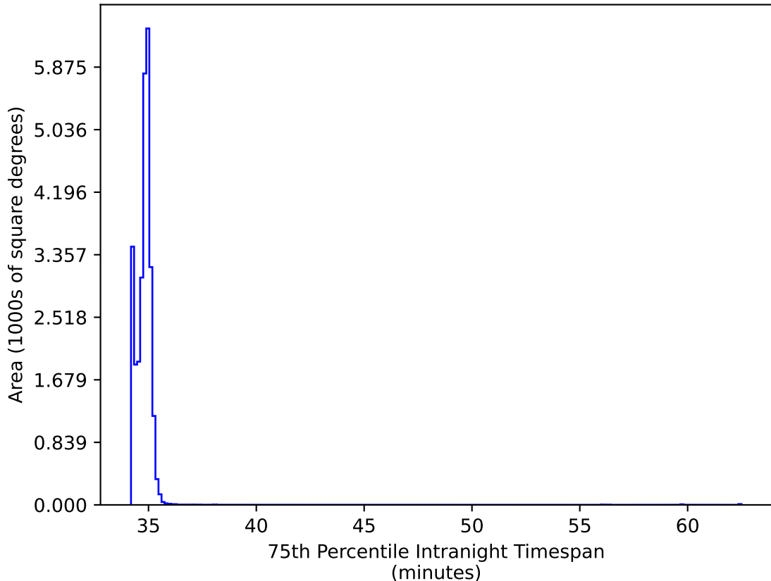
ddf_acor_sf15_lsf40_lsr10_v3.4_10yrs All sky all bands: 75th Percentile Intranight Timespan
