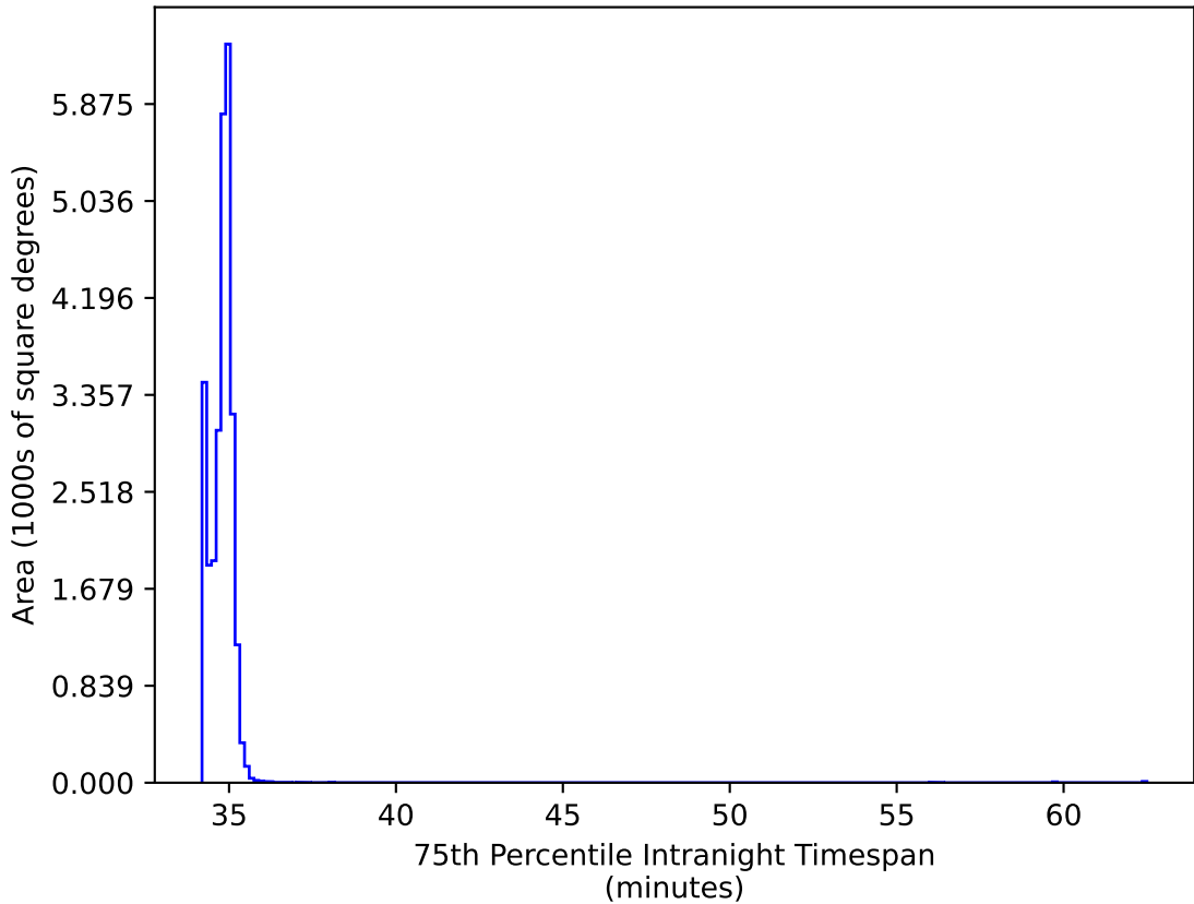
ddf_acor_sf15_lsf40_lsr10_v3.4_10yrs All sky: 75th Percentile Intranight Timespan
