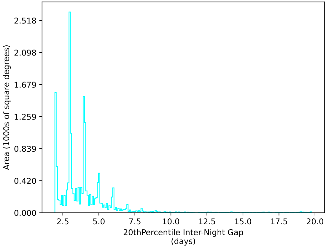
ddf_acor_sf15_lsf40_lsr10_v3.4_10yrs WFD u band: 20thPercentile Inter-Night Gap
