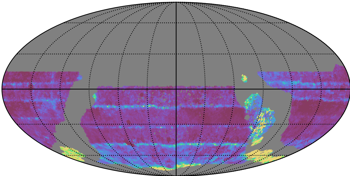
ddf_acor_sf15_lsf40_lsr10_v3.4_10yrs WFD all bands: 20thPercentile Inter-Night Gap
