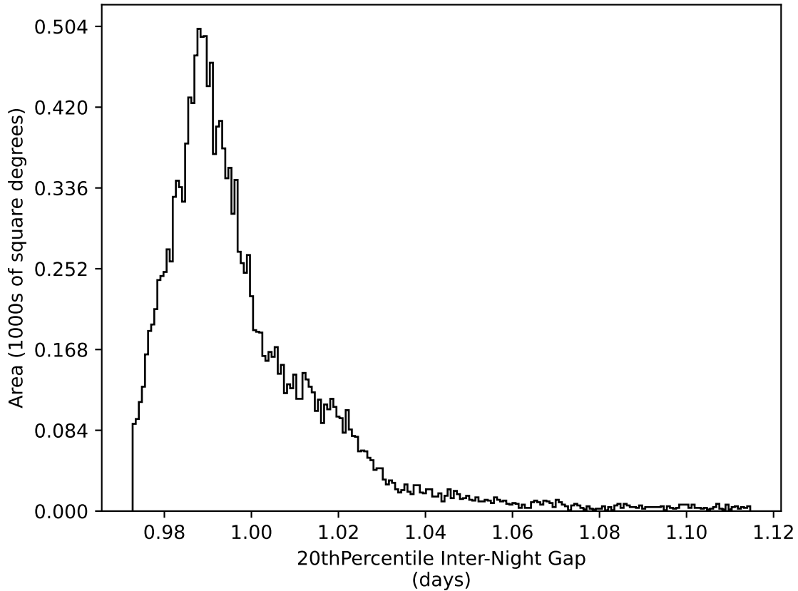
ddf_acor_sf15_ls40_lsr10_v3.4_10yrs WFD all bands: 20thPercentile Inter-Night Gap
