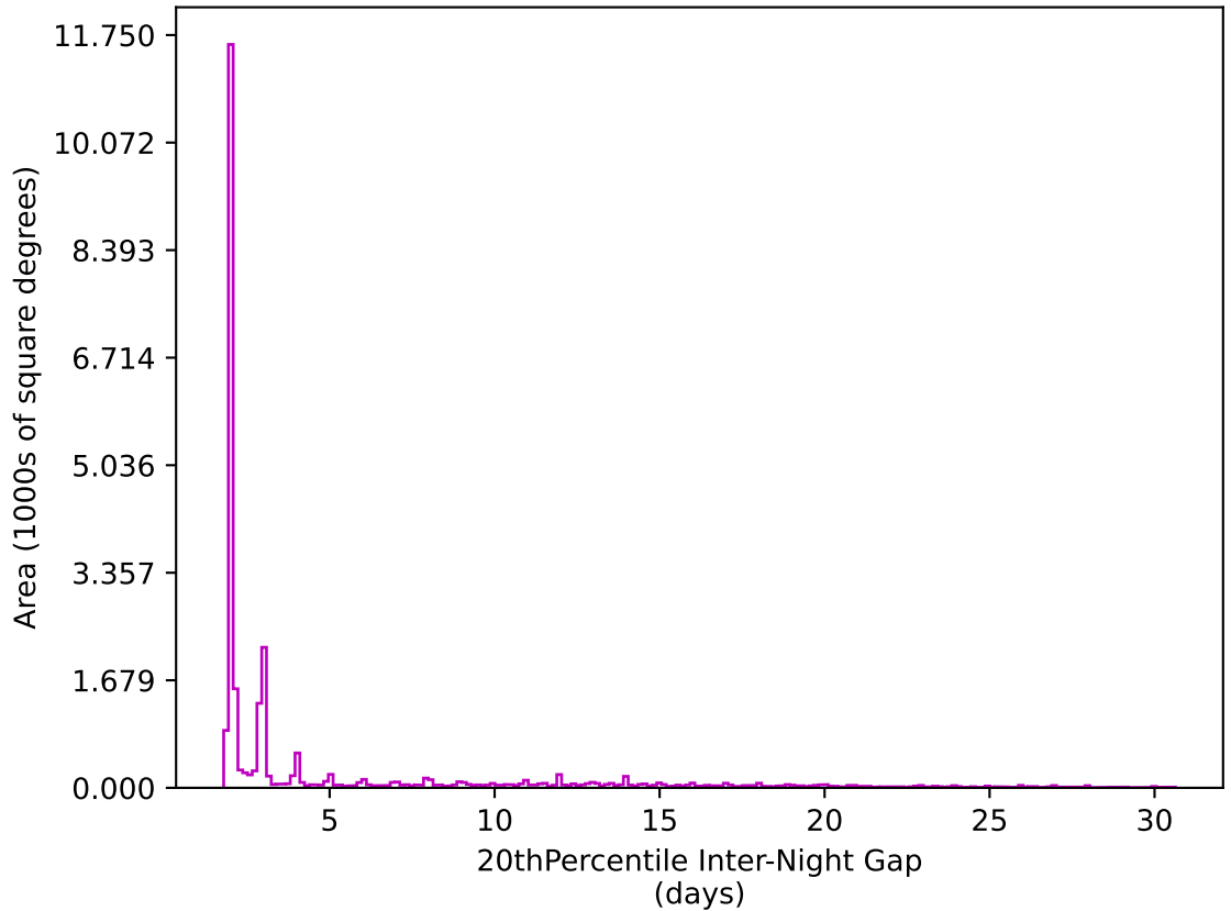
ddf_acor_sf15_ls40_lsr10_v3.4_10yrs All sky z band: 20thPercentile Inter-Night Gap
