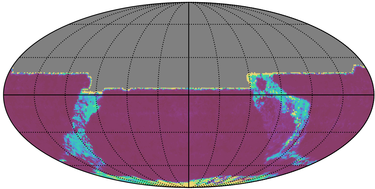
ddf_acor_sf15_lsf40_lsr10_v3.4_10yrs All sky y band: 20thPercentile Inter-Night Gap
