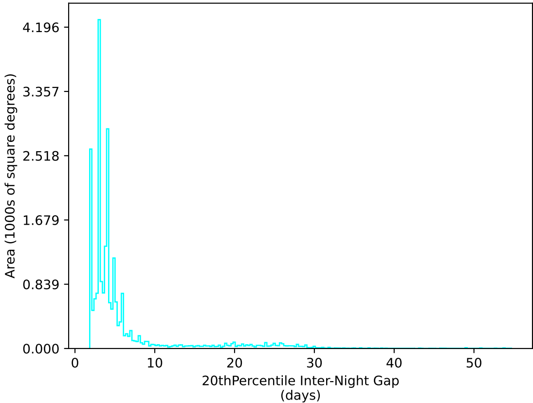
ddf_acor_sf15_ls40_lsr10_v3.4_10yrs All sky u band: 20thPercentile Inter-Night Gap
