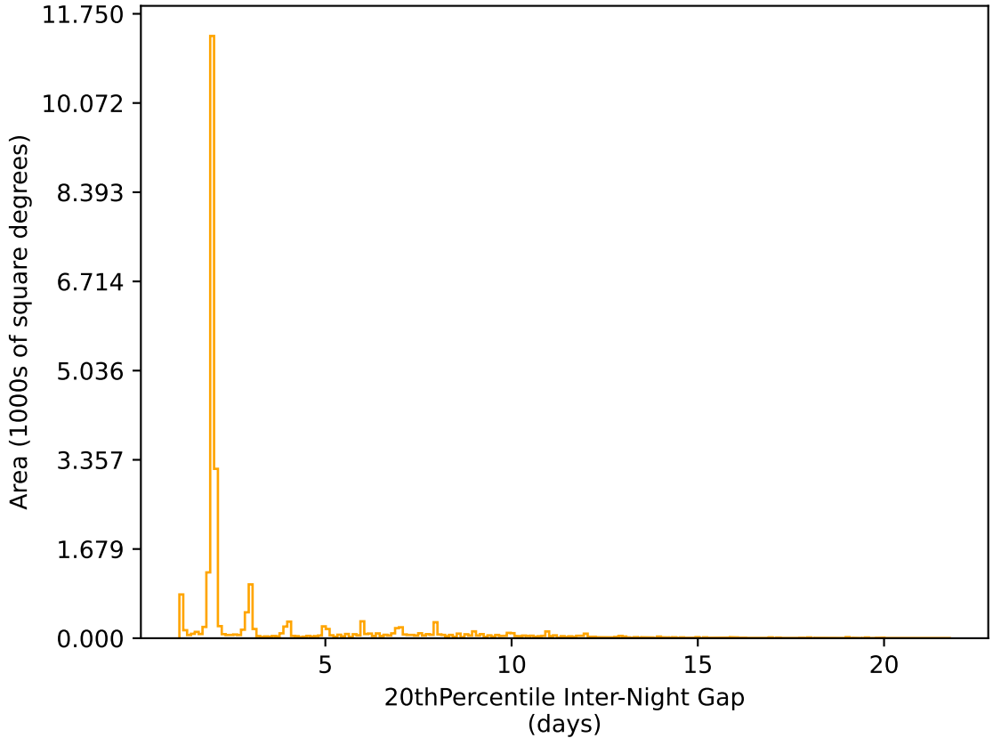
ddf_acor_sf15_lsf40_lsr10_v3.4_10yrs All sky r band: 20thPercentile Inter-Night Gap
