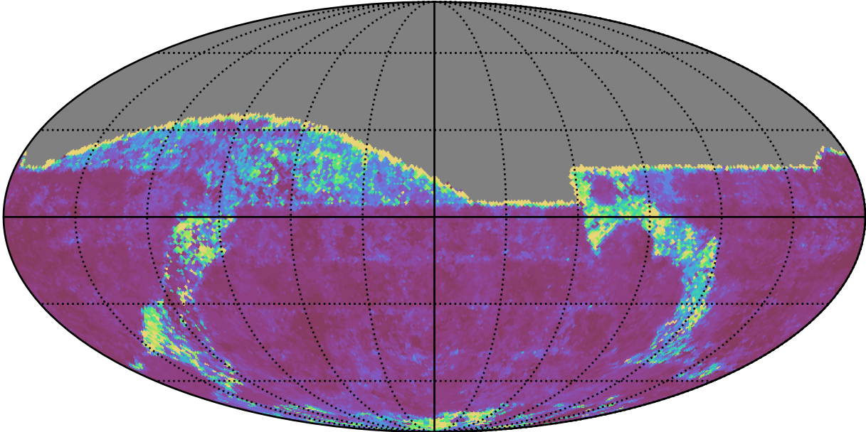
ddf_acor_sf15_lsf40_lsr10_v3.4_10yrs All sky g band: 20thPercentile Inter-Night Gap
