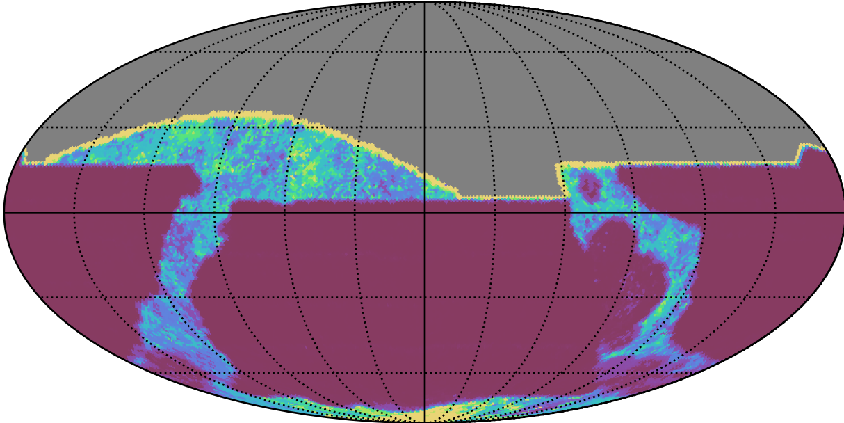
ddf_acor_sf15_lsf40_lsr10_v3.4_10yrs All sky all bands: 20thPercentile Inter-Night Gap
