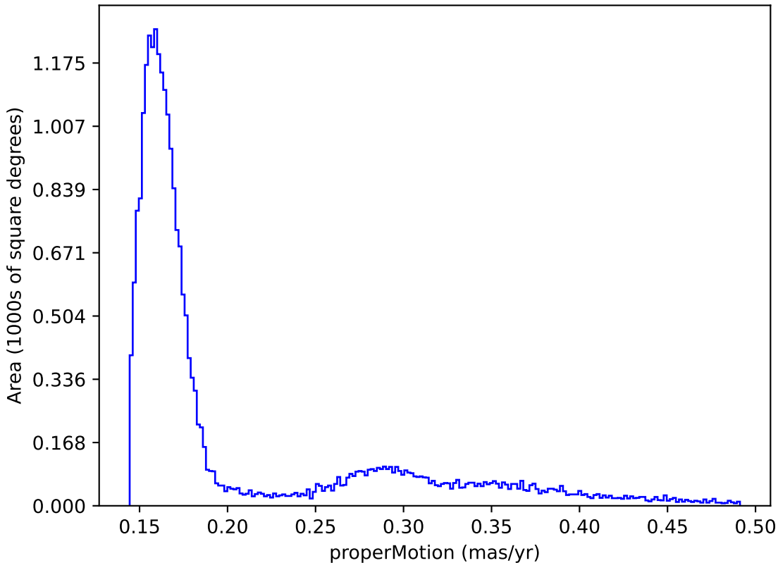
ddf_acor_sf15_lsf40_lsr10_v3.4_10yrs : properMotion
