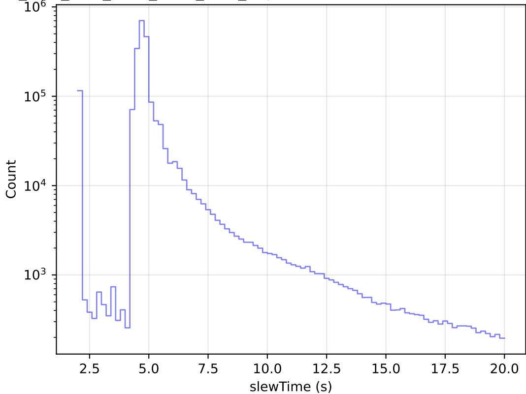
ddf_acor_sf15_Isf40_Isr10_v3.4_10yrs All visits: Zoom Slew Time Histogram
