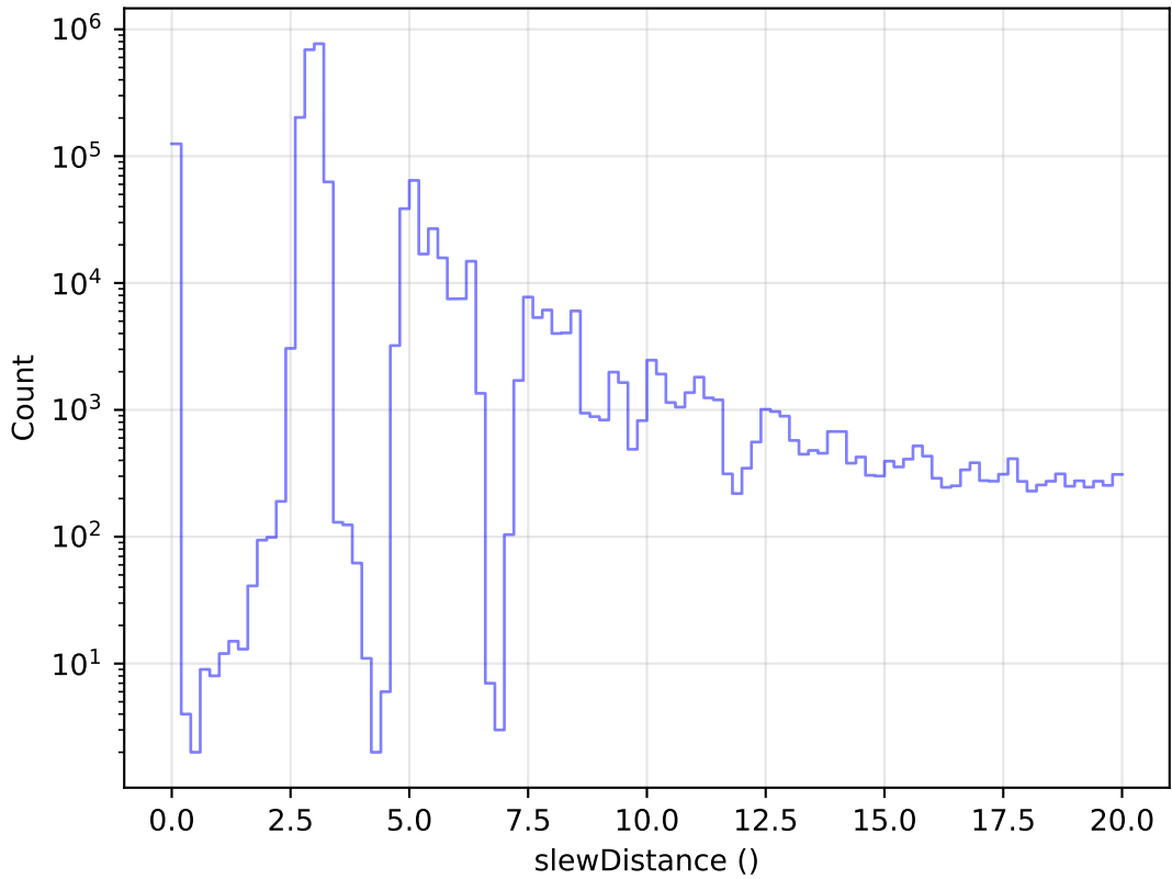
ddf_acor_sf15_lsf40_lsr10_v3.4_10yrs All visits: Zoom Slew Distance Histogram
