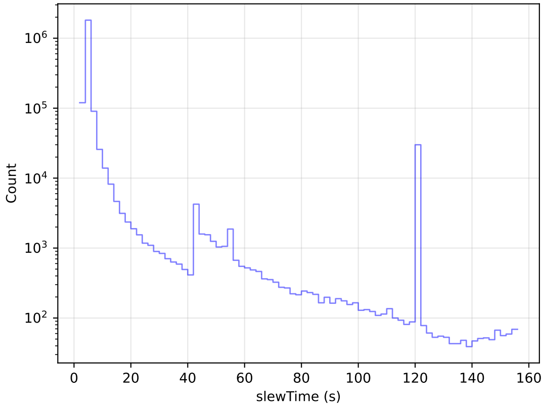
ddf_acor_sf15_lsf40_lsr10_v3.4_10yrs All visits: Slew Time Histogram
