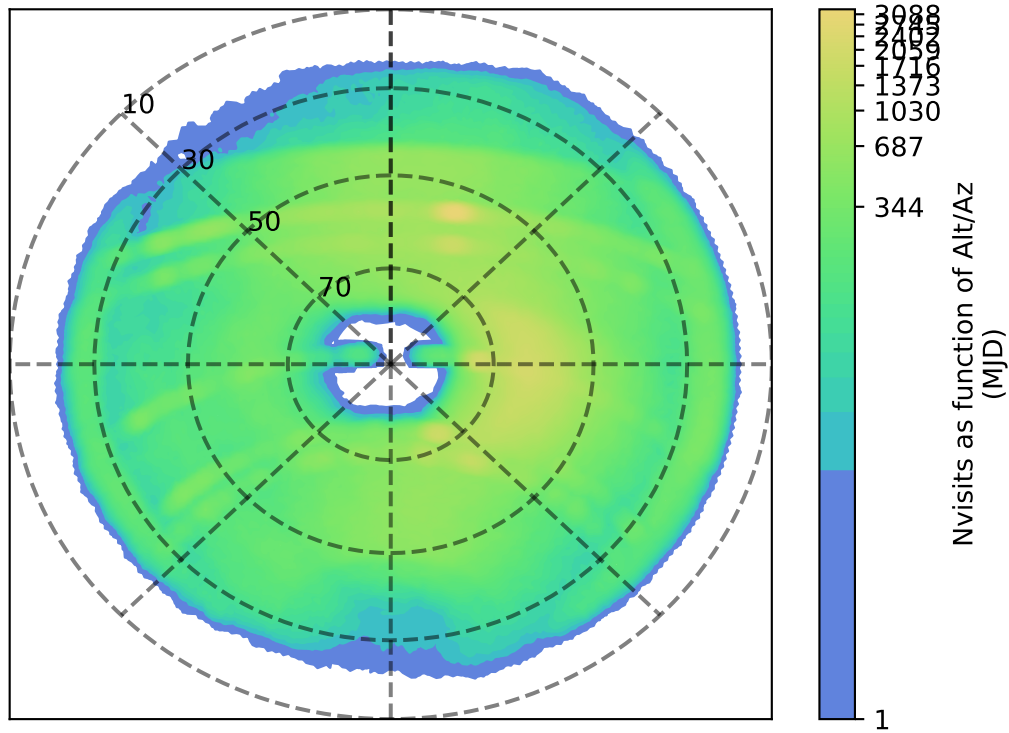
ddf_acor_sf15_lsf40_lsr10_v3.4_10yrs z: Nvisits as function of Alt/Az
