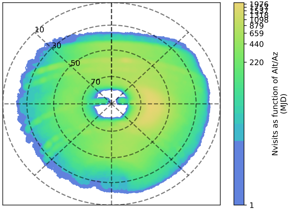
ddf_acor_sf15_lsf40_lsr10_v3.4_10yrs y: Nvisits as function of Alt/Az
