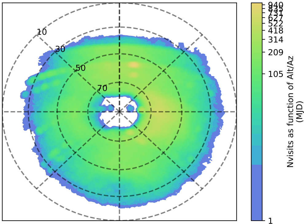
ddf_acor_sf15_lsf40_lsr10_v3.4_10yrs u: Nvisits as function of Alt/Az
