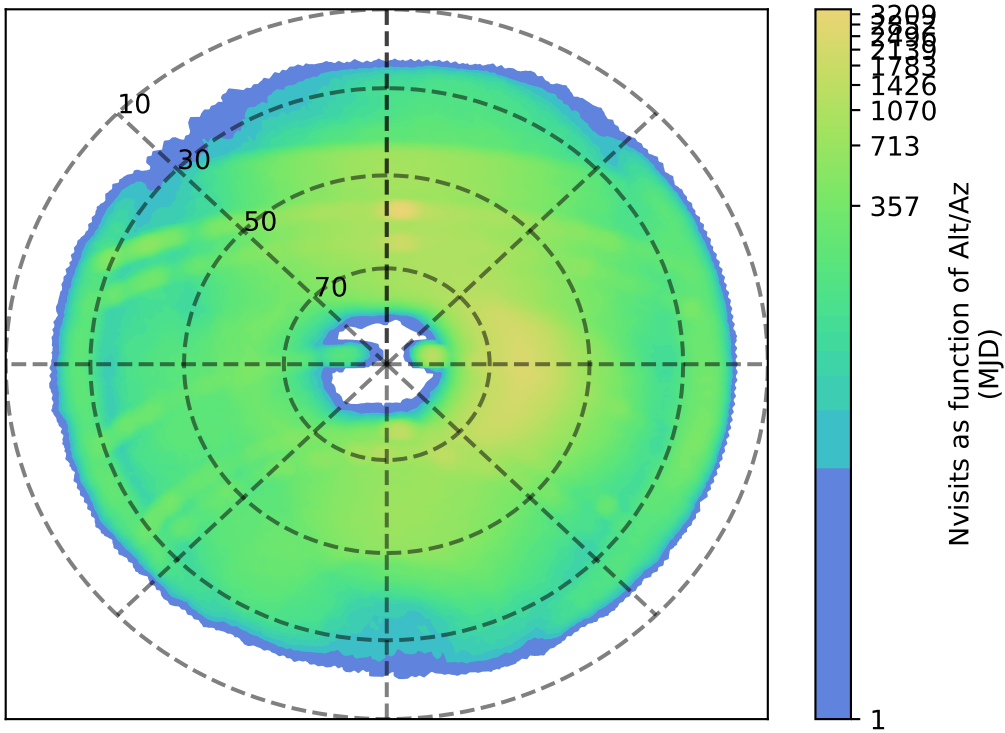
ddf_acor_sf15_ls40_lsr10_v3.4_10yrs i: Nvisits as function of Alt/Az
