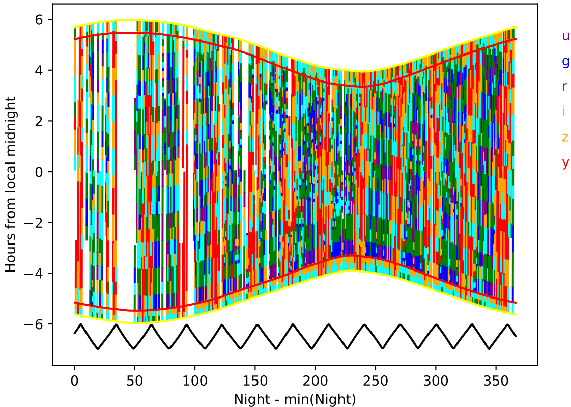
ddf_acor_sf15_lsf40_lsr10_v3.4_10yrs year 6-7: Hourglass
