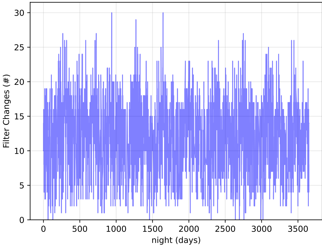
ddf_acor_sf15_lsf40_lsr10_v3.4_10yrs : Filter Changes
