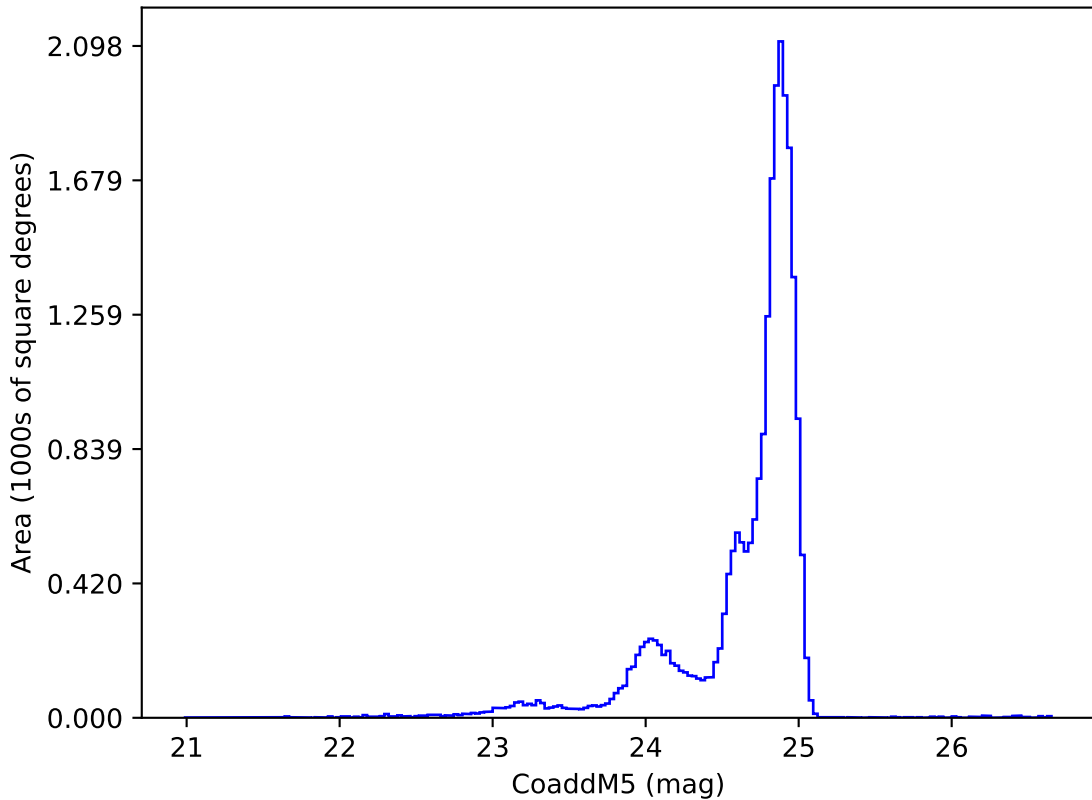
ddf_acor_sf15_lsf40_lsr10_v3.4_10yrs y: CoaddM5
