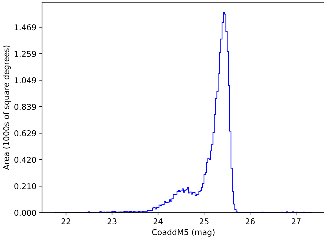
ddf_acor_sf15_lsf40_lsr10_v3.4_10yrs u: CoaddM5
