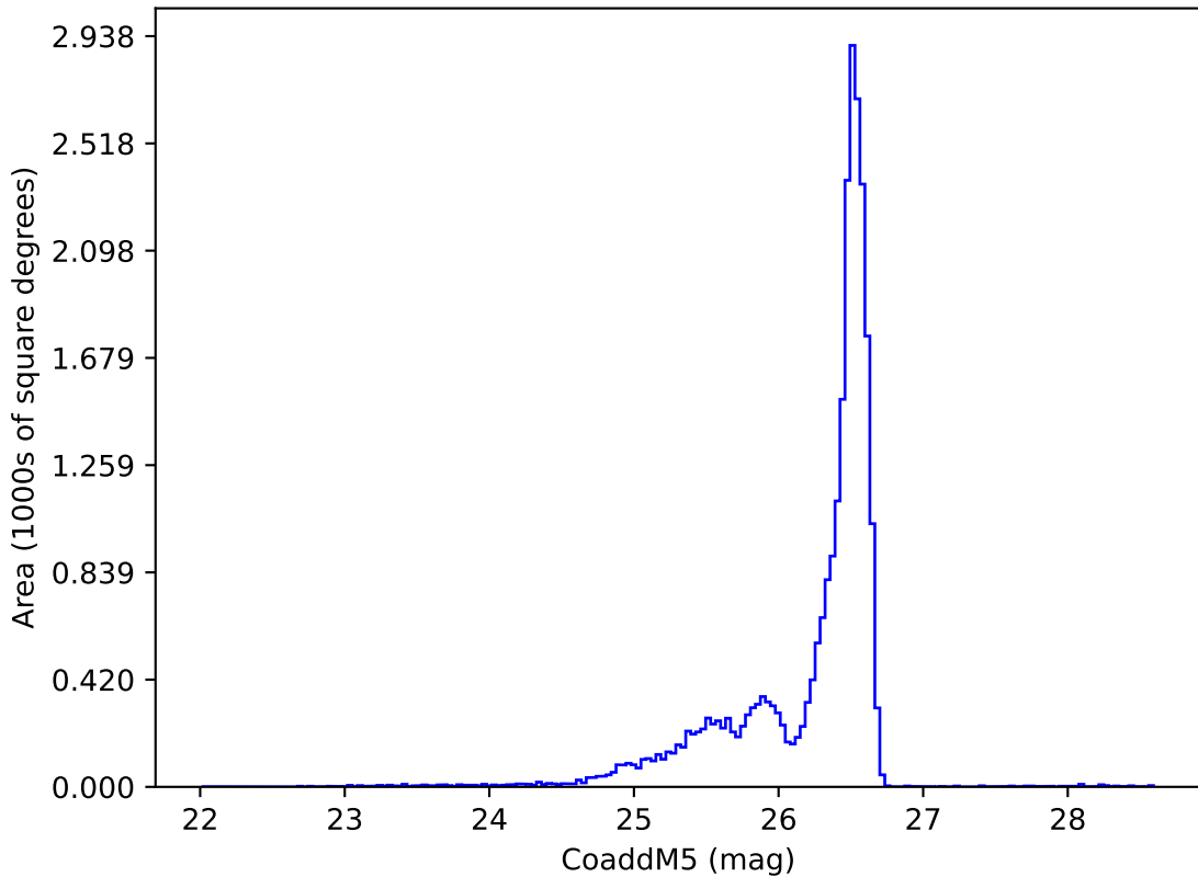
ddf_acor_sf15_lsf40_lsr10_v3.4_10yrs i: CoaddM5
