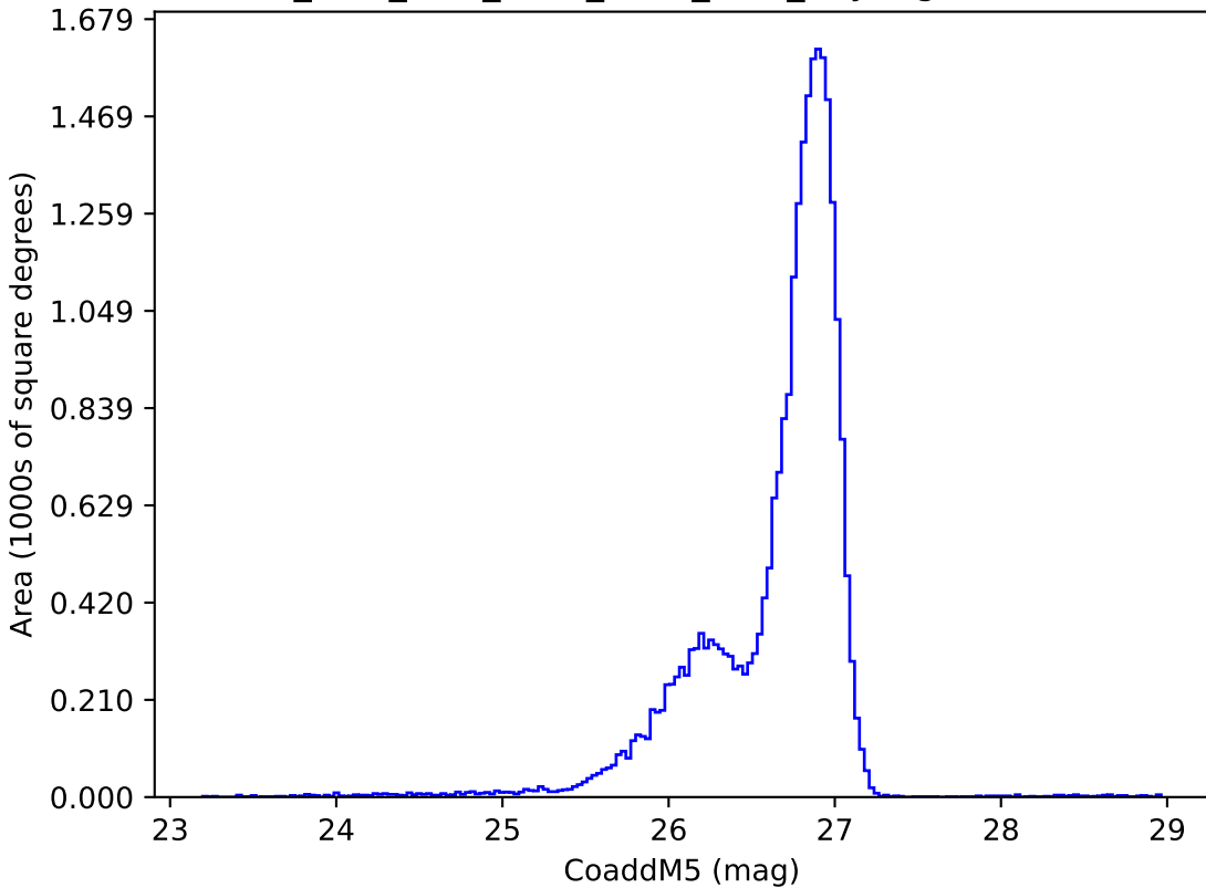
ddf_acor_sf15_lsf40_lsr10_v3.4_10yrs g: CoaddM5
