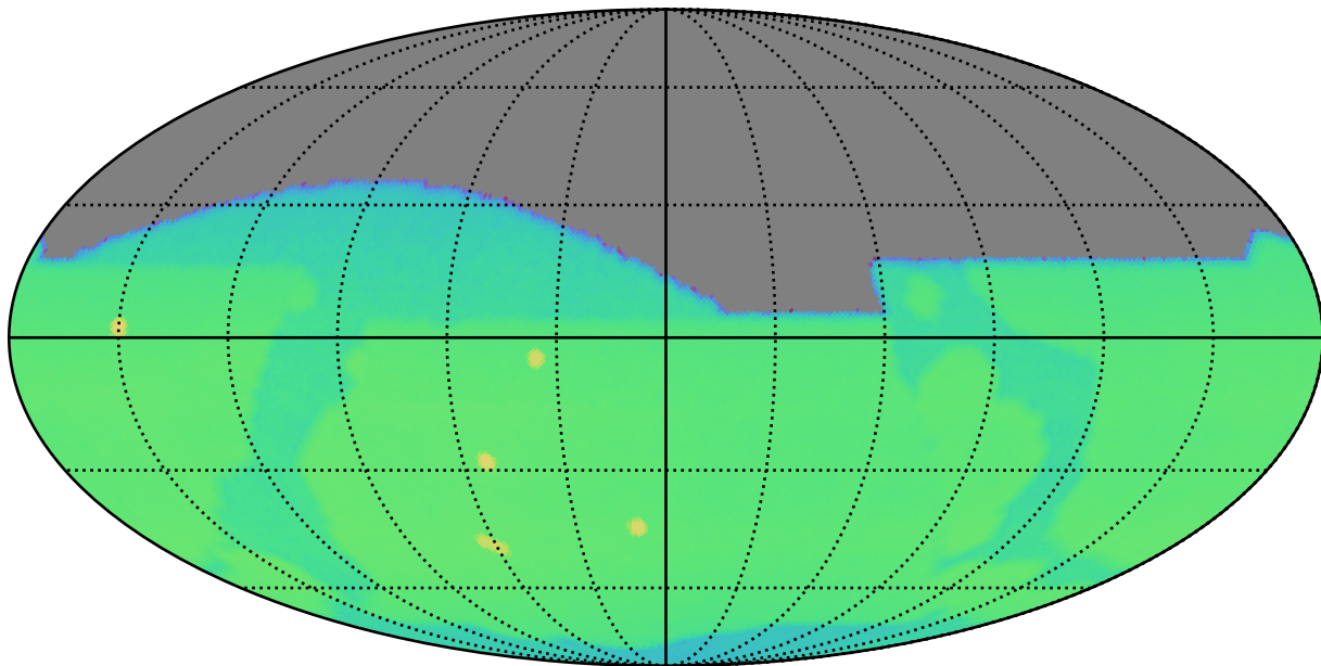
ddf_acor_sf15_lsf40_lsr10_v3.4_10yrs : CoaddM5
