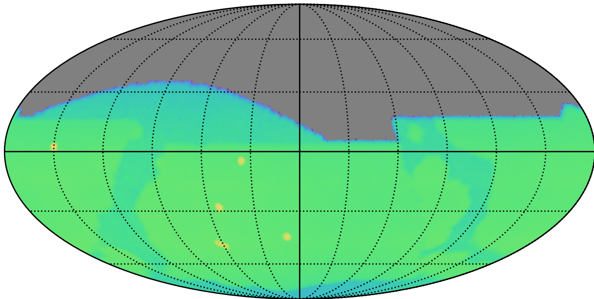
ddf_acor_sf15_lsf40_lsr10_v3.4_10yrs : CoaddM5
